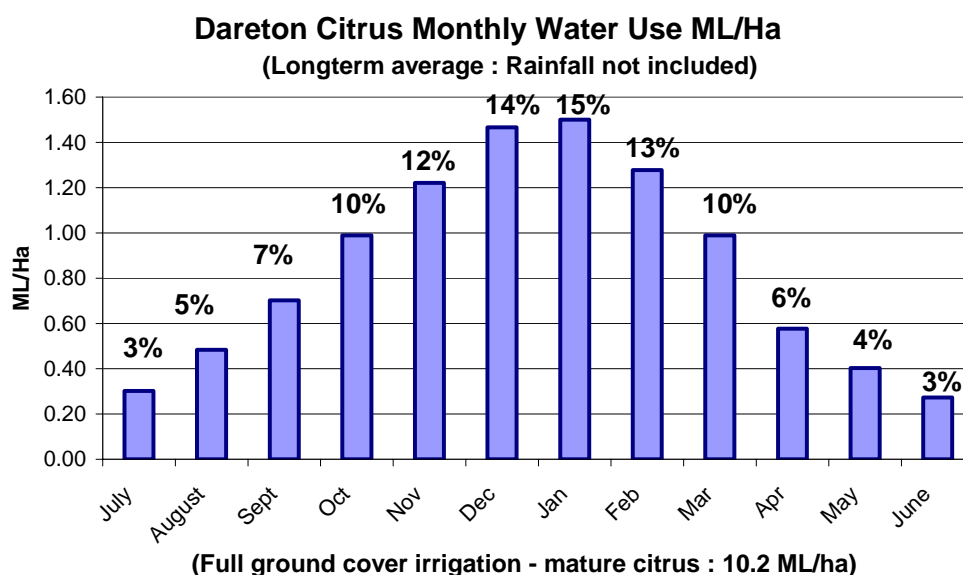
Figure 1: Long-term average water use of mature citrus trees with full ground cover, sprinkler irrigation and monthly percentage values at Dareton.
